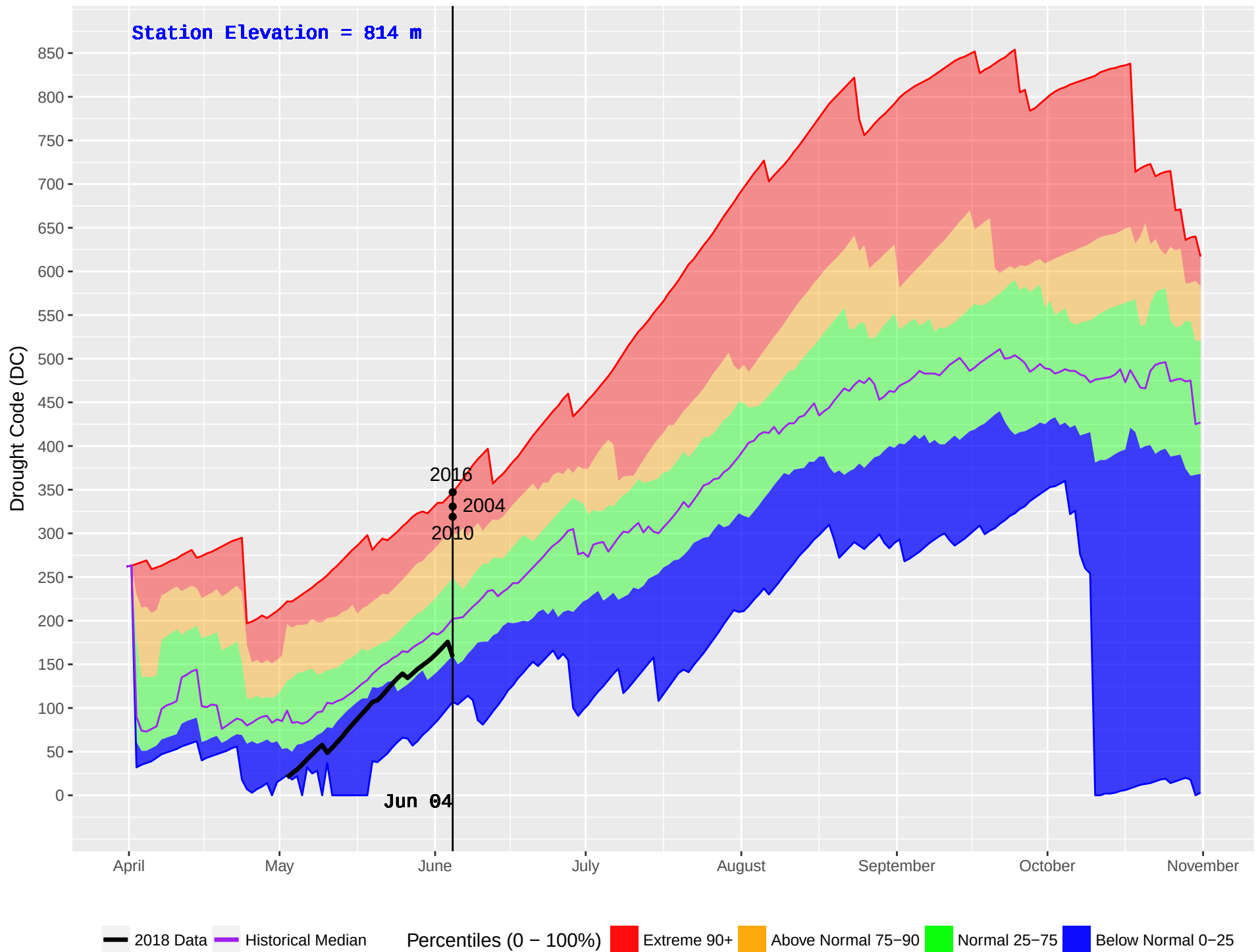
CHILAKO (189) : Historical (1986–2016) and Current (2018) Noon Drought Code (DC)
