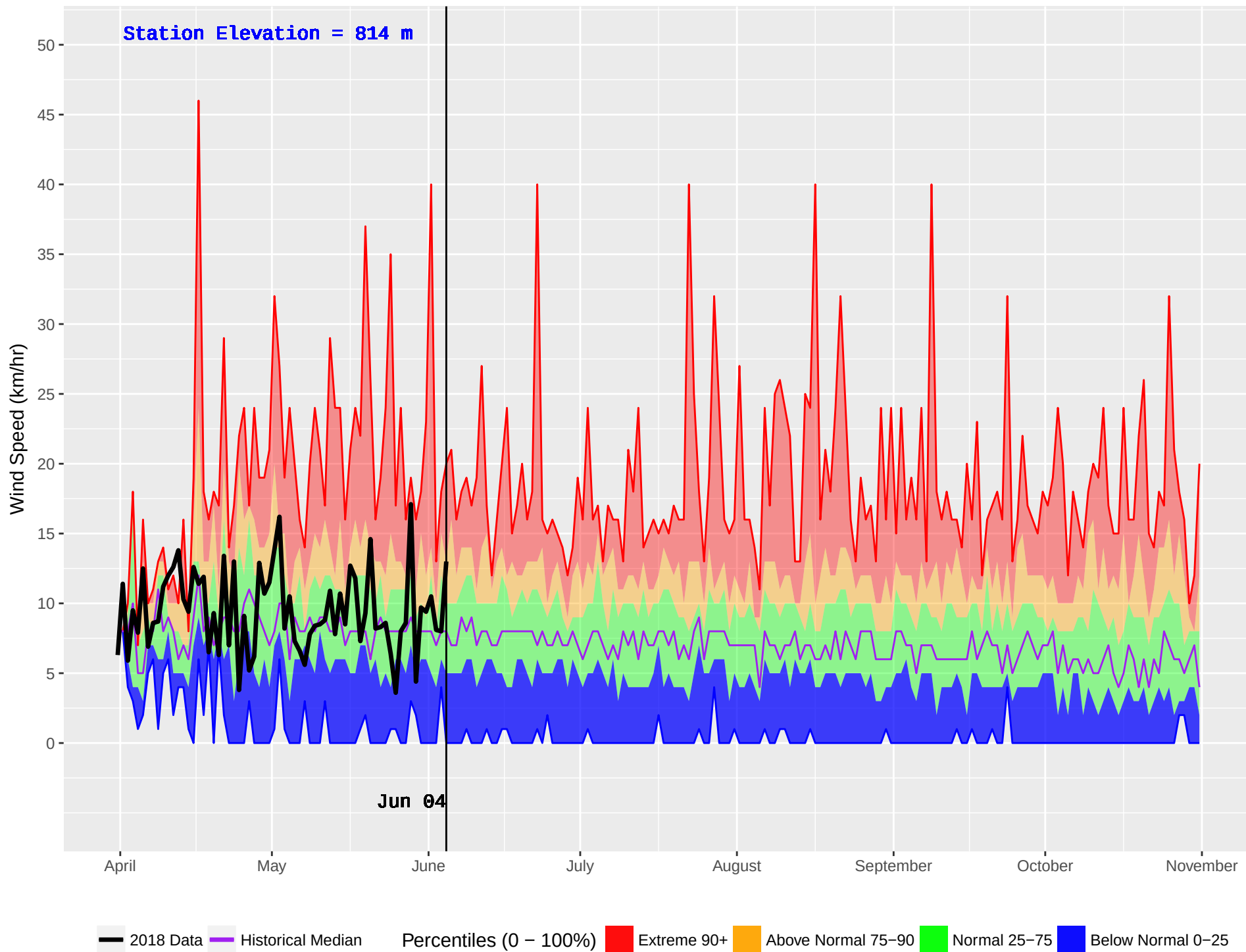
CHILAKO (189) : Historical (1986–2016) and Current (2018) Noon Wind Speed
