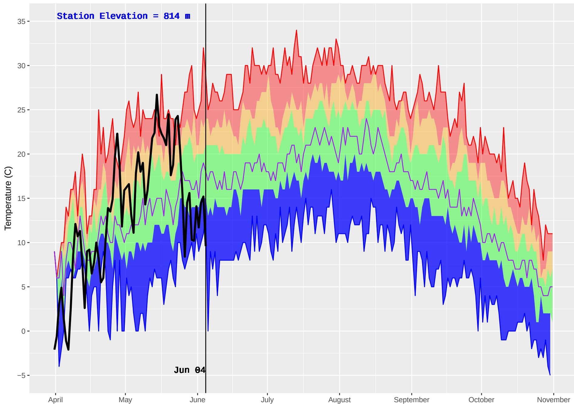
CHILAKO (189) : Historical (1986–2016) and Current (2018) Noon Temperature
