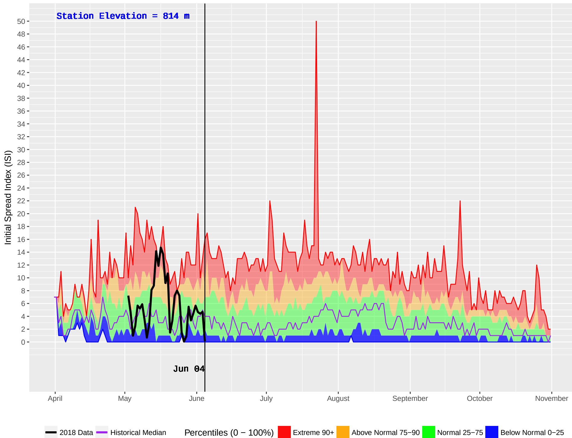
CHILAKO (189) : Historical (1986–2016) and Current (2018) Noon Initial Spread Index (ISI)
