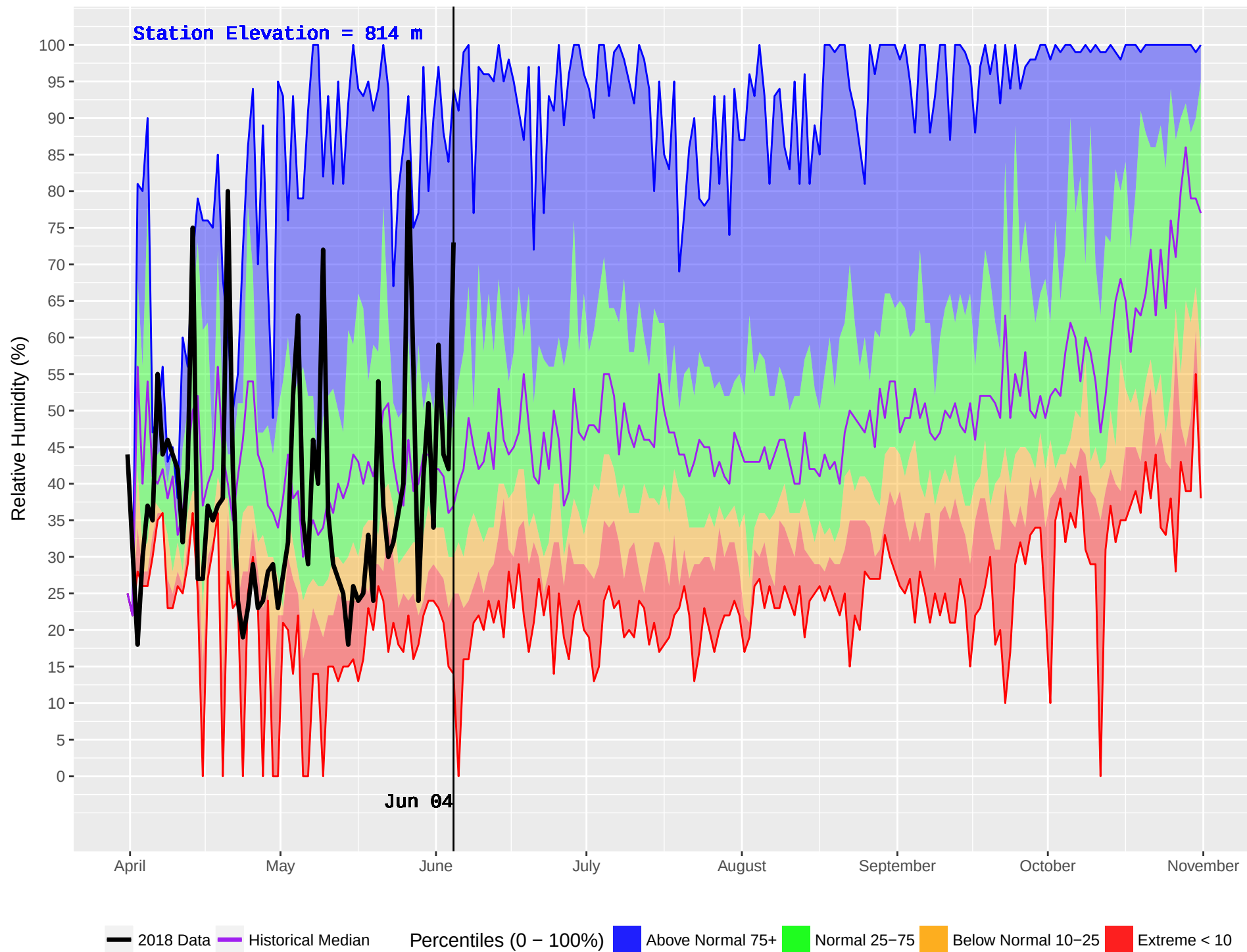
CHILAKO (189) : Historical (1986–2016) and Current (2018) Noon Relative Humidity
