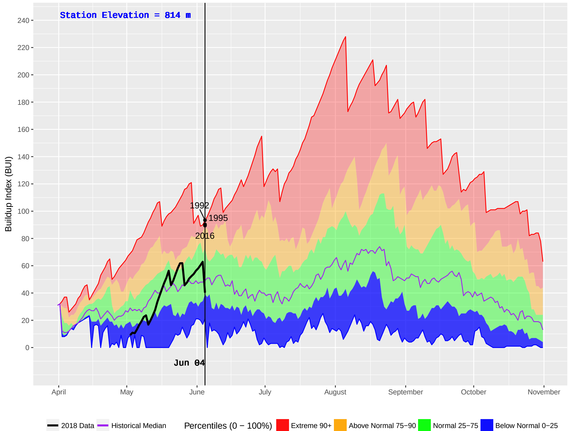
CHILAKO (189) : Historical (1986–2016) and Current (2018) Noon Buildup Index (BUI)
